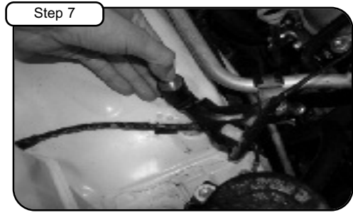
Step 7 With 10mm socket and extension, remove bolt holding AC bracket. Insert M8 isolation mount and hand tighten firmly. (It may be necessary to clean the threads of undercoating or paint)
