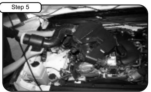
Step 5 Disconnect vacuum and valve cover vent line. Remove OE intake out of vehicle. (Remove and save the two OE rubber grommets & spacers that hold in airbox from step 3)
