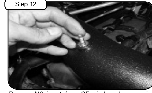
Step 12 Remove M6 insert from OE air box, loosen using adjustable wrench. Re-install on to new tube and tighten. Connect large vent hose and connect small vent hose (5/32" hose provided) between tube and fuel regulator.
