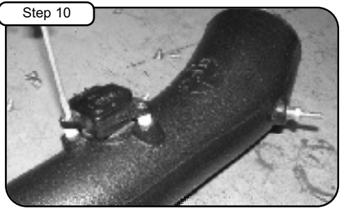
Step 10 Remove MAF sensor from OE airbox using phillips screwdriver. Re-install to new aFe tube with hardware provided using flat head screwdriver (make sure gasket and nylon spacers are between tube and sensor). Install brass hose fitting.
