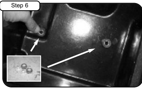
Step 6 With grommets removed from OE intake, place onto new housing with metal spacers.
