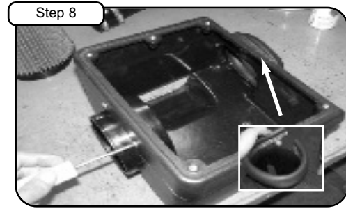
Step 8 Place intake adaptor into housing. Use M6 button head screws provided to attach adaptor and tighten using 5/32" allen wrench. Place 3/4" trim seal onto side vent of housing.
