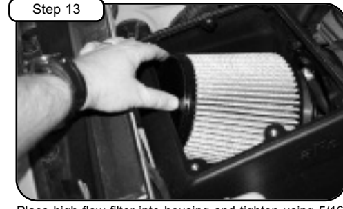
Step 13 Place high flow filter into housing and tighten using 5/16" nut driver. Place cover onto housing using M6 button head screws provided, tighten using 5/32" allen wrench. (Place filter into housing at slight angle)
