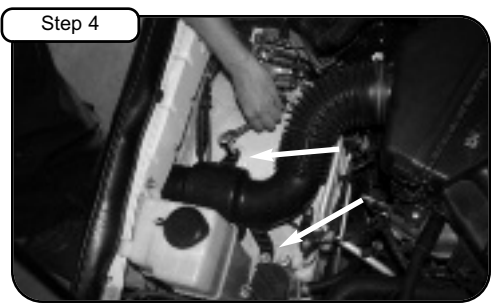
Step 4 With 12mm socket, loosen the two bolts holding in OE intake snorkel.
