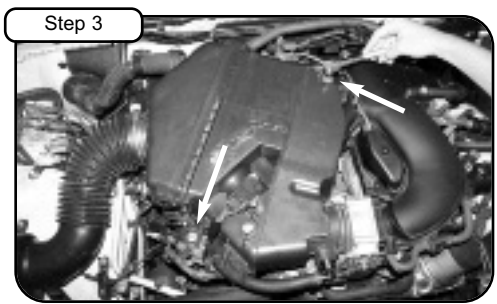
Step 3 Remove engine cover with 10mm socket. With 10mm socket remove the 2 bolts holding in OE airbox. Disconnect the MAF sensor.
